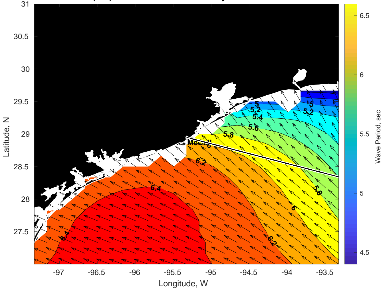
Wave Period (sec) for Brooks McCall at 02-May-2024 12:00:00
